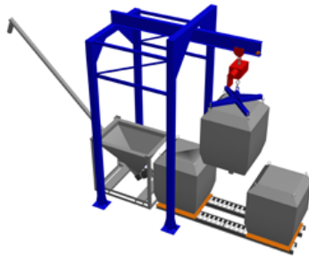
10' Bulk Bag Gantry
