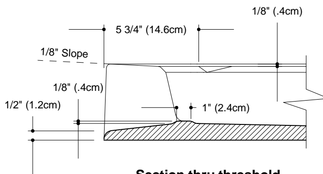
Section thru threshold Not to scale
