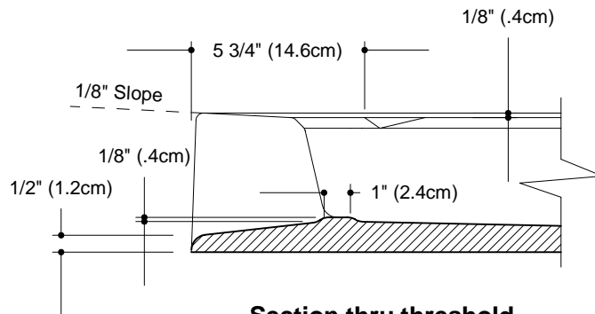
Section thru threshold Not to scale
